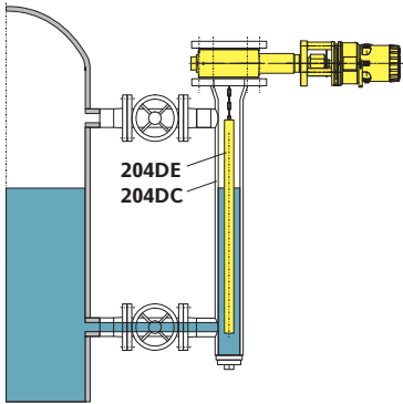
Mounted e.g. at side of vessel, with displacer chamber 204DE and displacer 204DC
