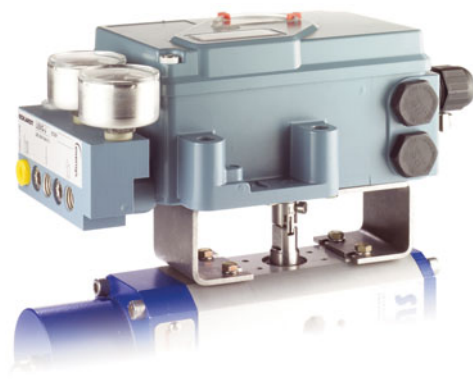
Example for mounting on rotary actuators.
